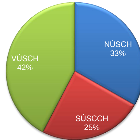
AFL
